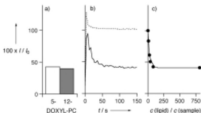
Figure 2. Fluorescence quenching of the emission intensity of oligo( p -phenylene) 1 in spin-labeled EYPC-SUVs ( \lambda_{\text{ex}} = 328 nm, \lambda_{\text{em}} = 390 nm, 10 mM potassium phosphate buffer, 100 mM KCl, pH 6.4). a) Emission intensities ( I/I_0 ) of 1 (100 nM) with 0.25 mM of EYPC-SUVs containing 8.7% 5- and 12-DOXYL-PC ( I ) relative to identical measurements with unlabeled EYPC-SUVs ( I_0 ). b) Time course of the emission intensity of 1 (100 nM) after addition to 0.25 mM of unlabeled (---) and 12-DOXYL-PC-labeled EYPC-SUVs (—). c) Dependence of the quenching of 1 by 12-DOXYL-PC as a function of lipid/rod ratio at constant lipid concentration. [29]
